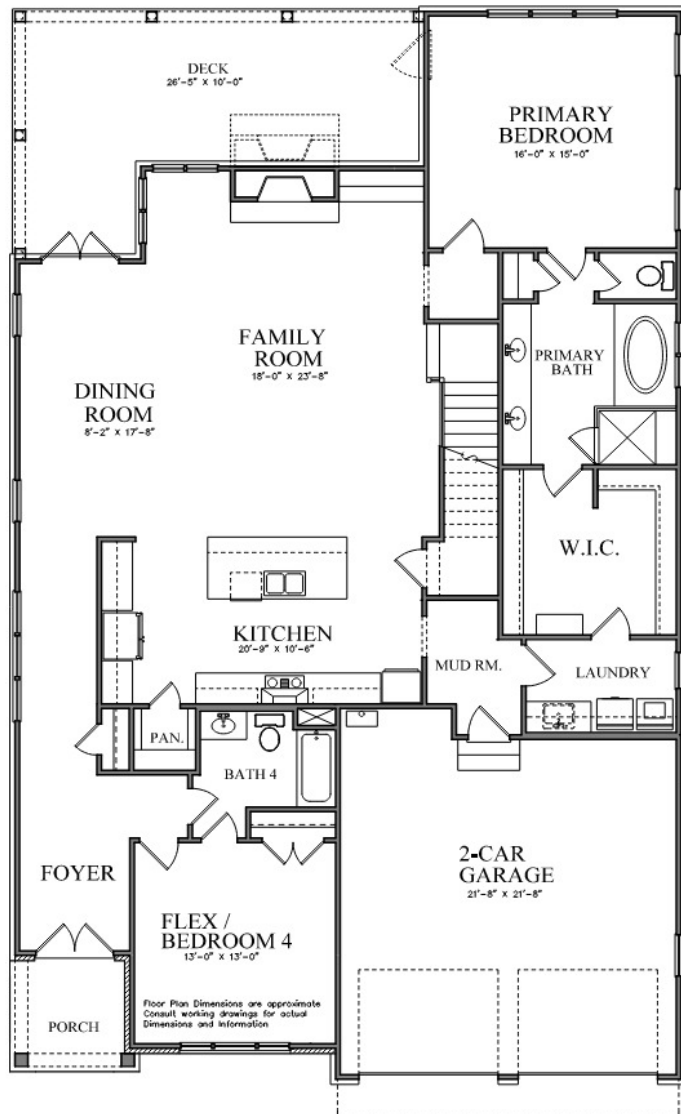
FIRST FLOOR PLAN TRENTON D
