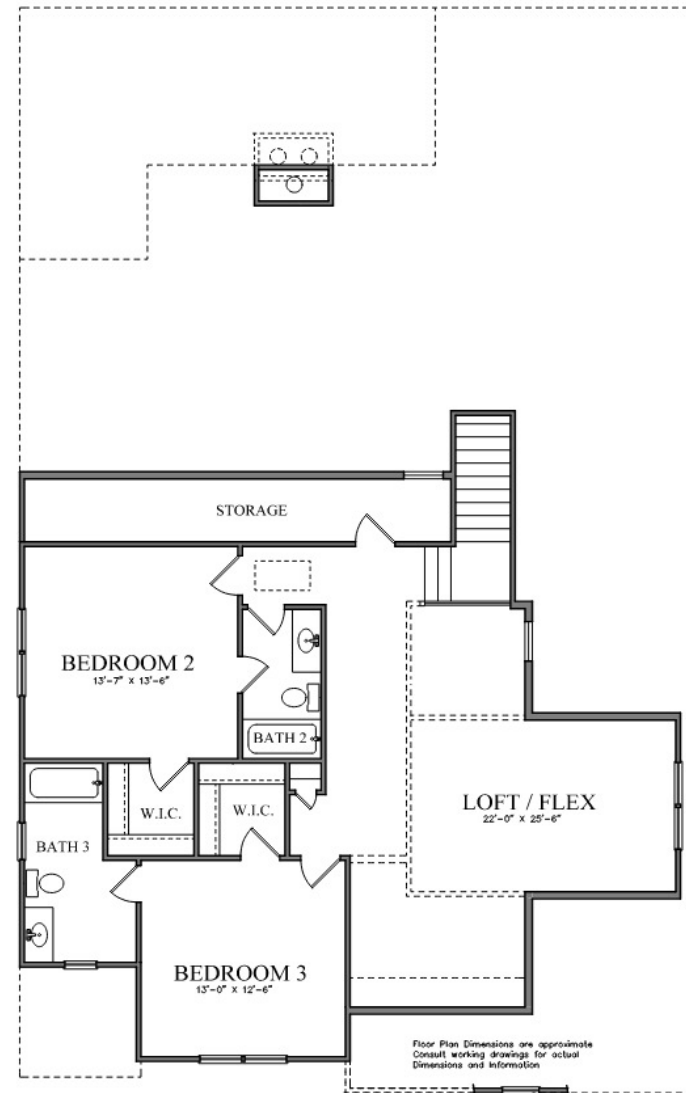
SECOND FLOOR PLAN TRENTON D
