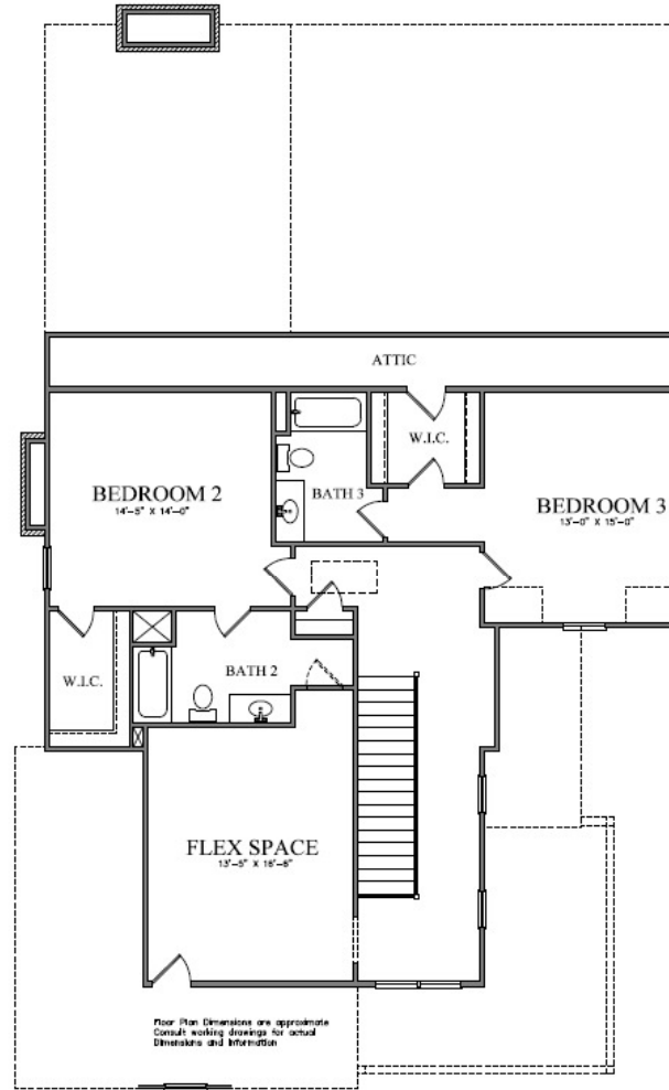
SECOND FLOOR PLAN WESTON D
