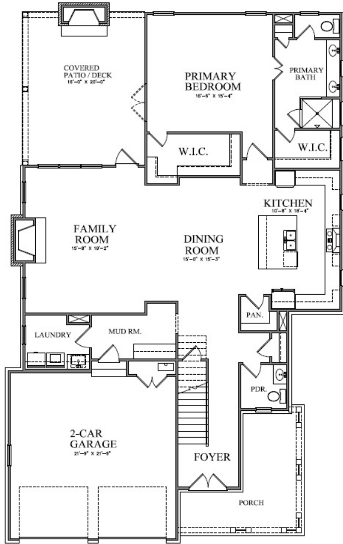
FIRST FLOOR PLAN WESTON D
