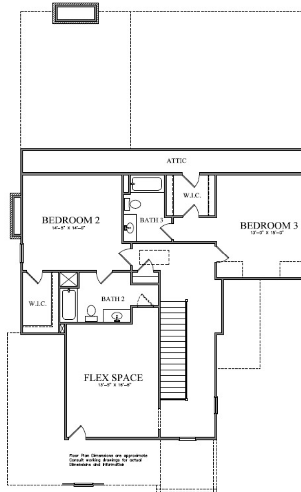
SECOND FLOOR PLAN WESTON E
