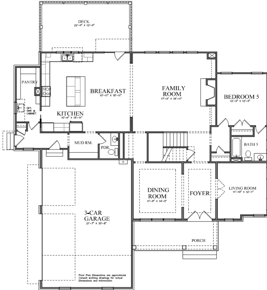
FIRST FLOOR PLAN OXFORD C
