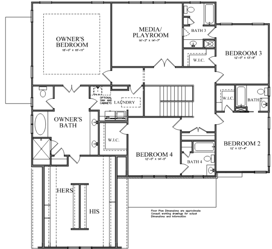
SECOND FLOOR PLAN OXFORD C
