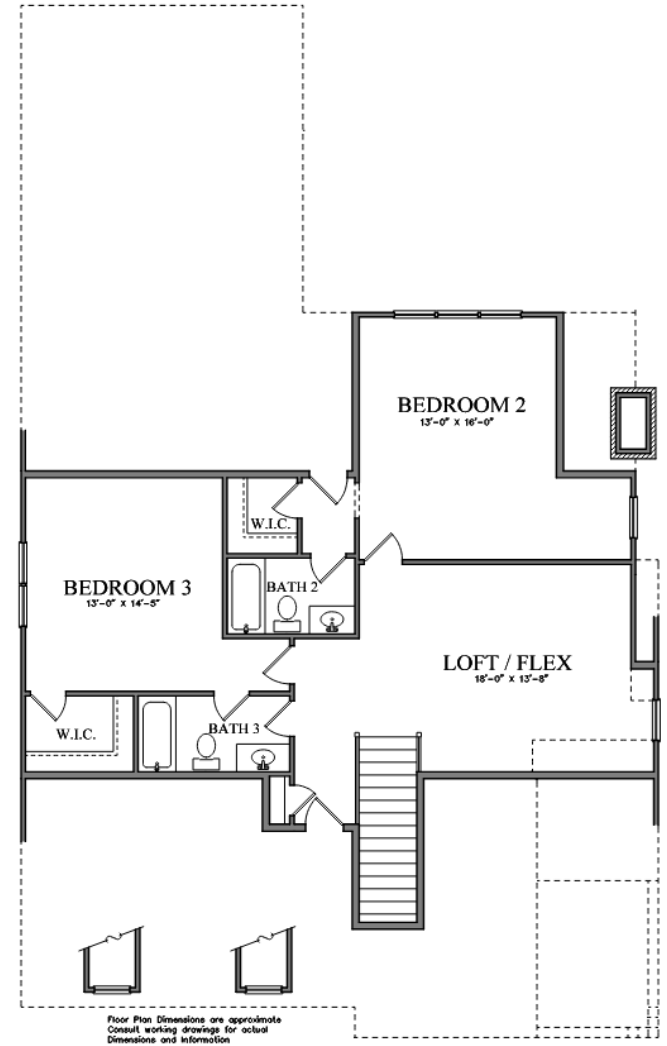
SECOND FLOOR PLAN OXFORD C
