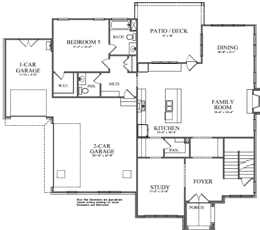
FIRST FLOOR PLAN ASHBURN A
