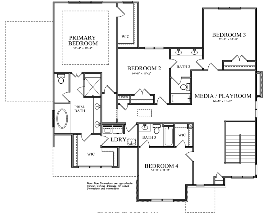
SECOND FLOOR PLAN ASHBURN A
