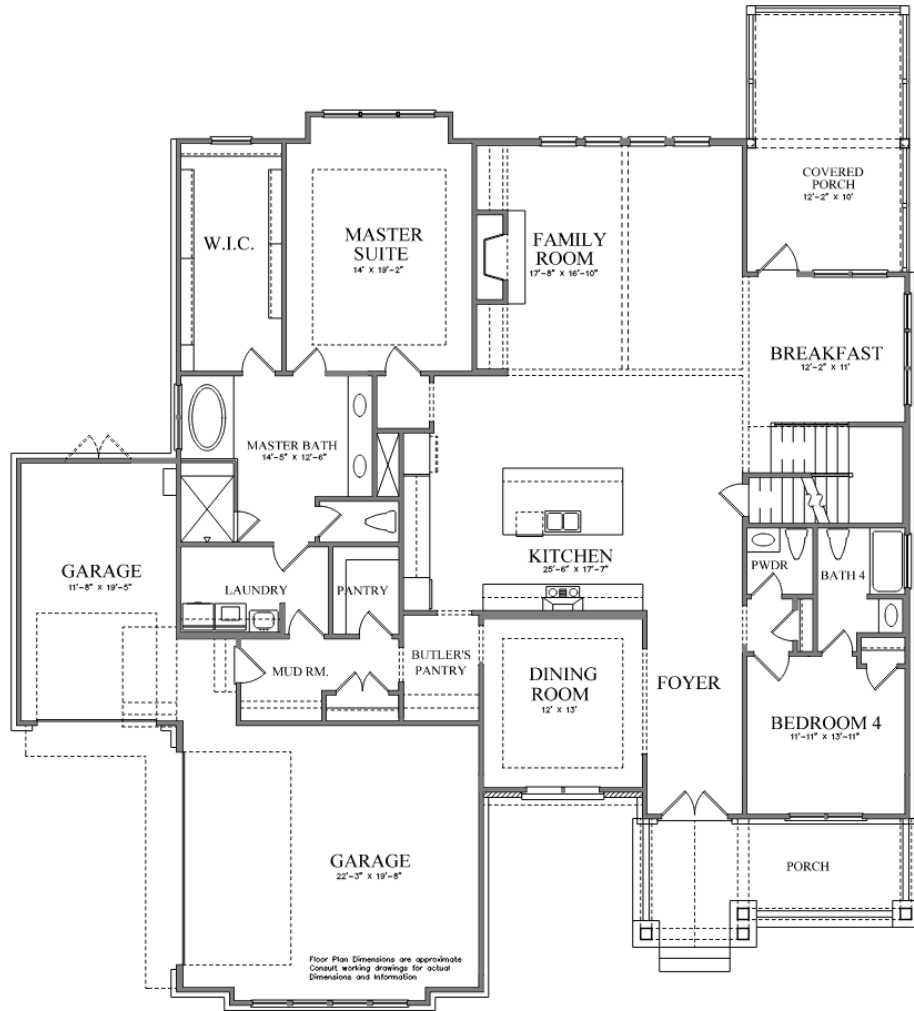
FIRST FLOOR PLAN EVANS B
