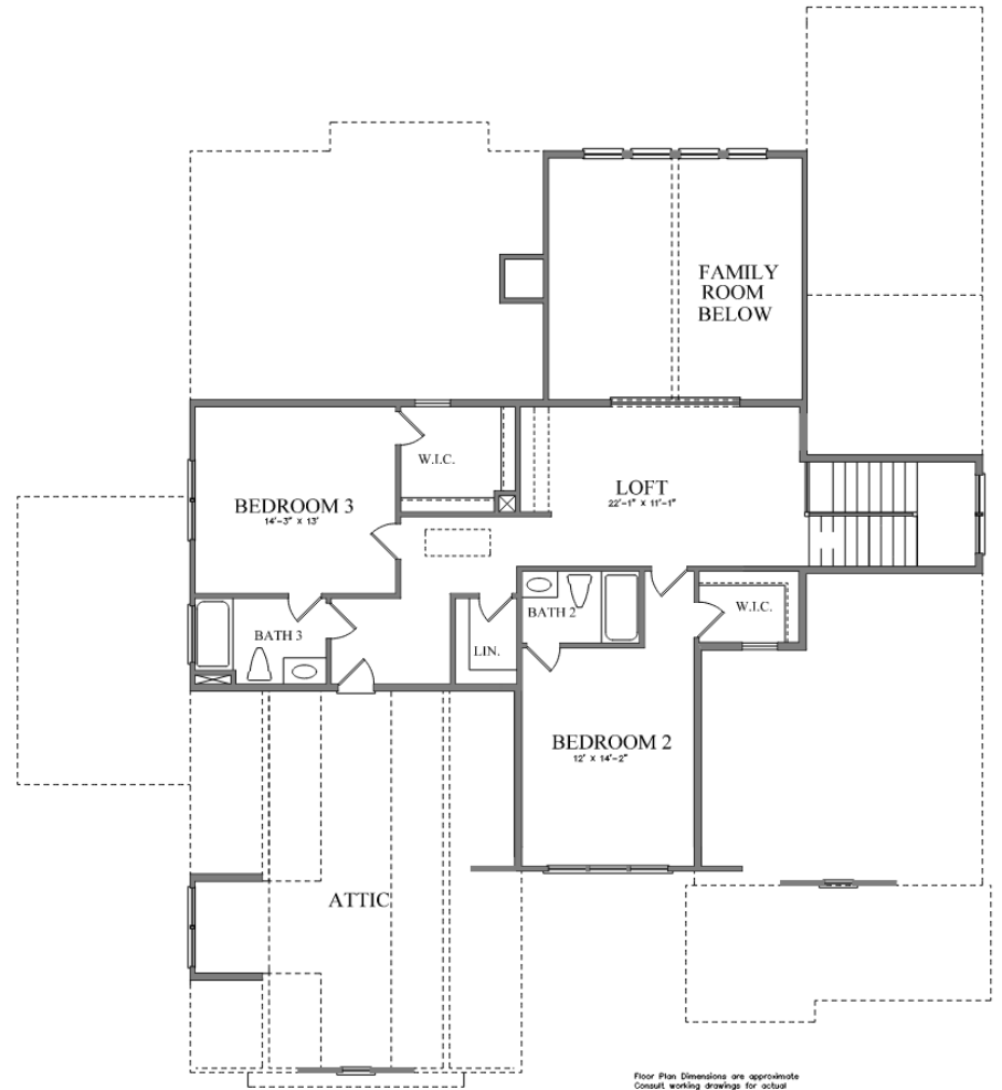
SECOND FLOOR PLAN EVANS B
