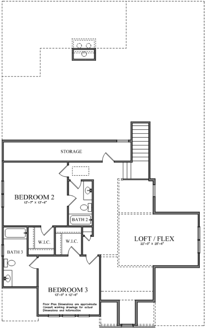
SECOND FLOOR PLAN TRENTON F
