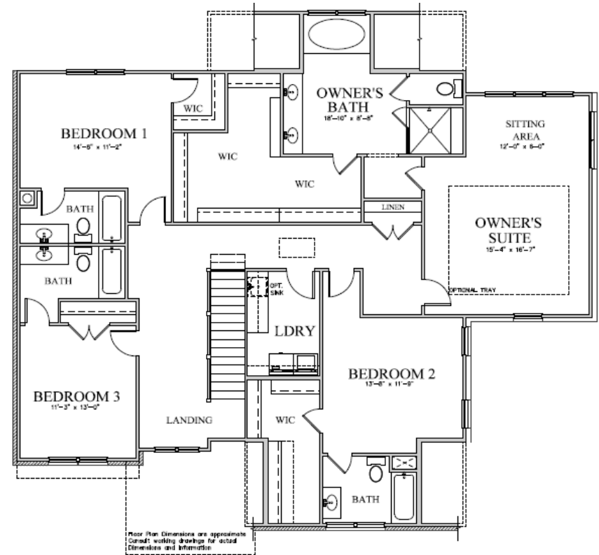
SECOND FLOOR PLAN BROOKS A
