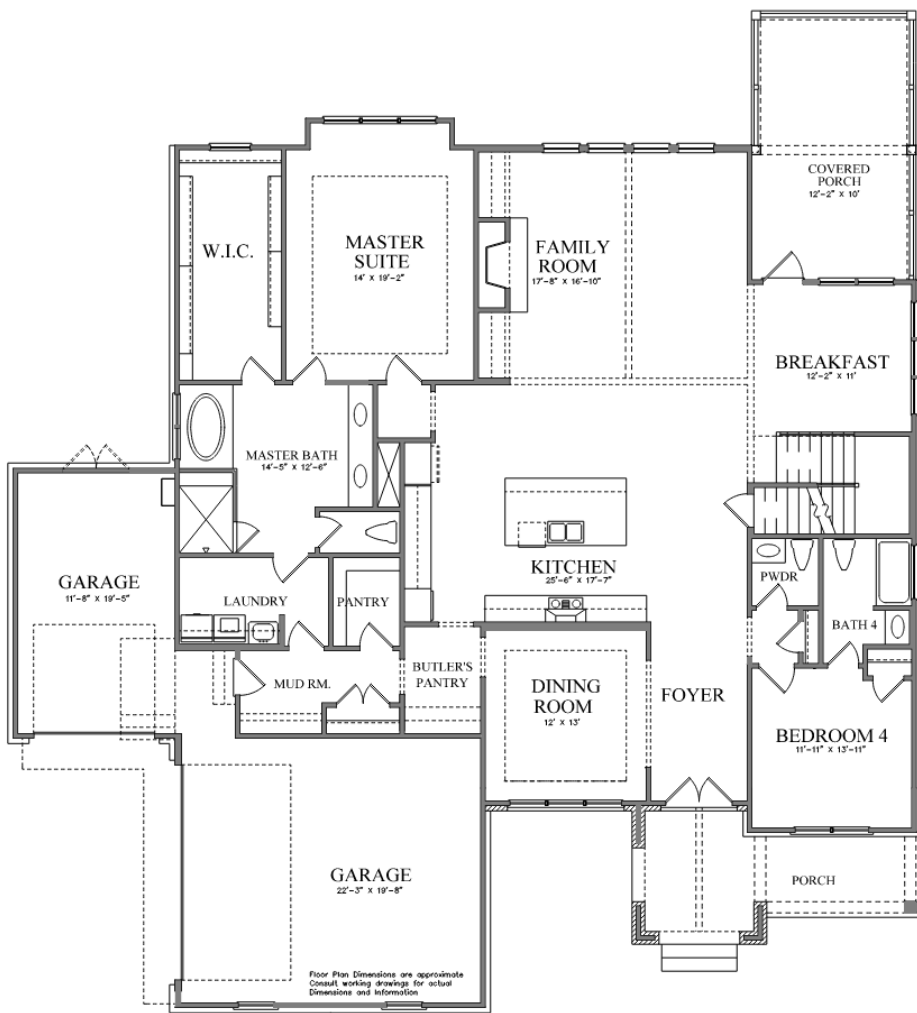
FIRST FLOOR PLAN EVANS E
