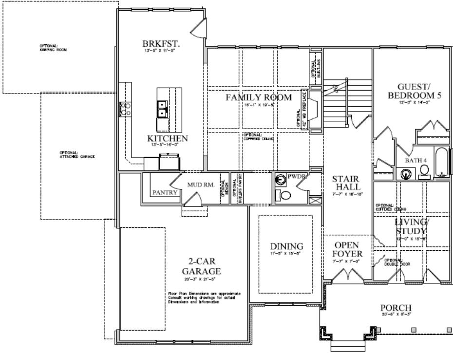
FIRST FLOOR PLAN DILLARD C
