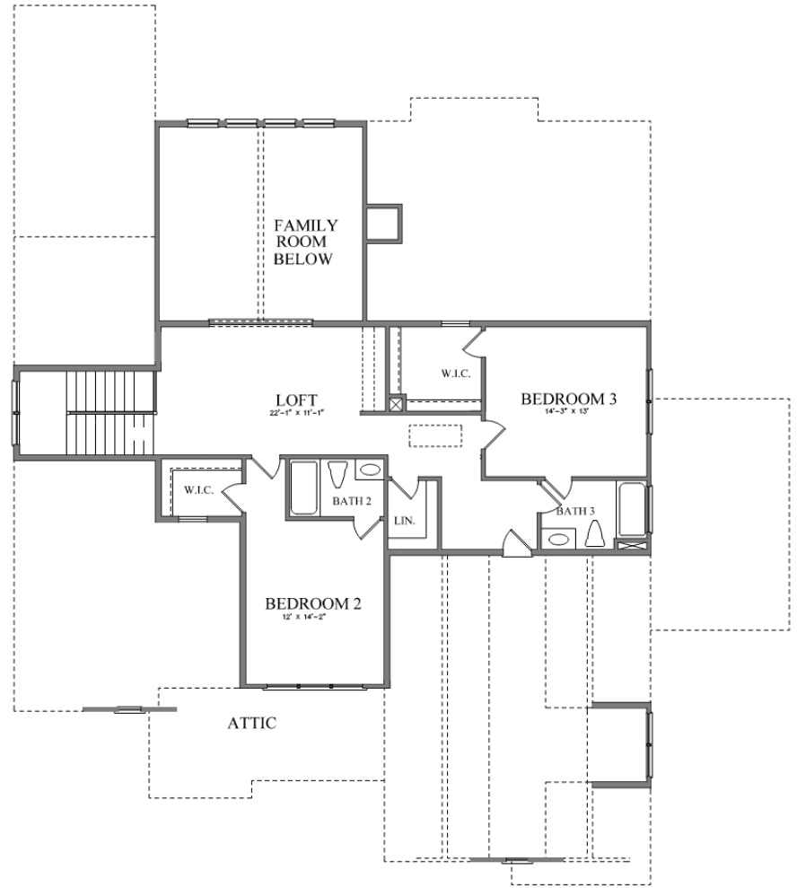
SECOND FLOOR PLAN EVANS A
