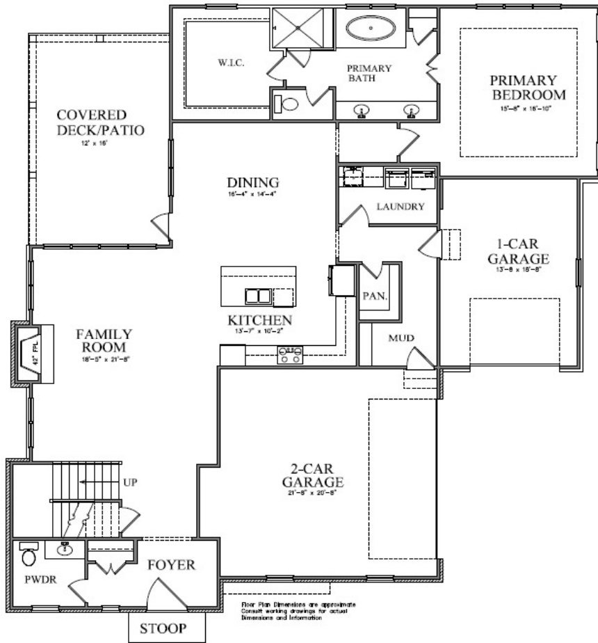
FIRST FLOOR PLAN DESOTO A
