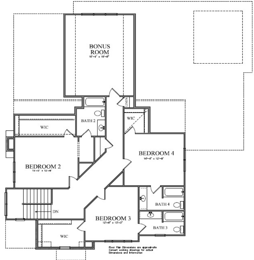
SECOND FLOOR PLAN DESOTO A
